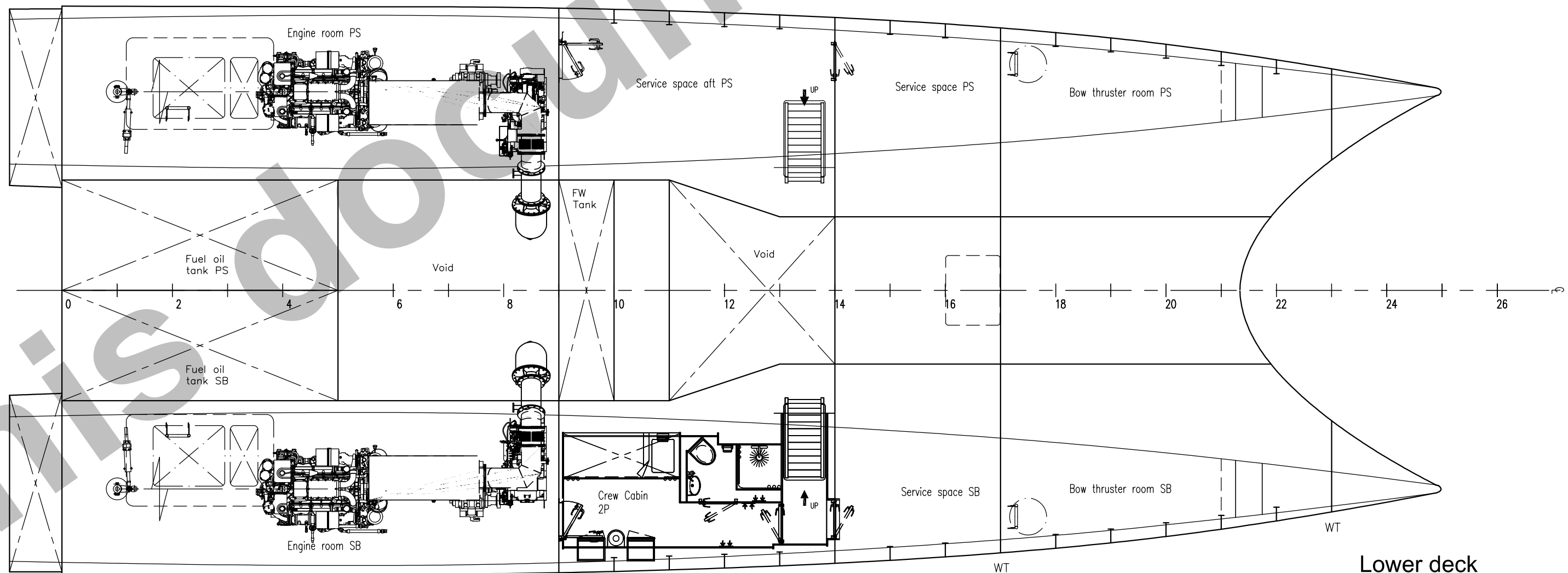
Lower deck
