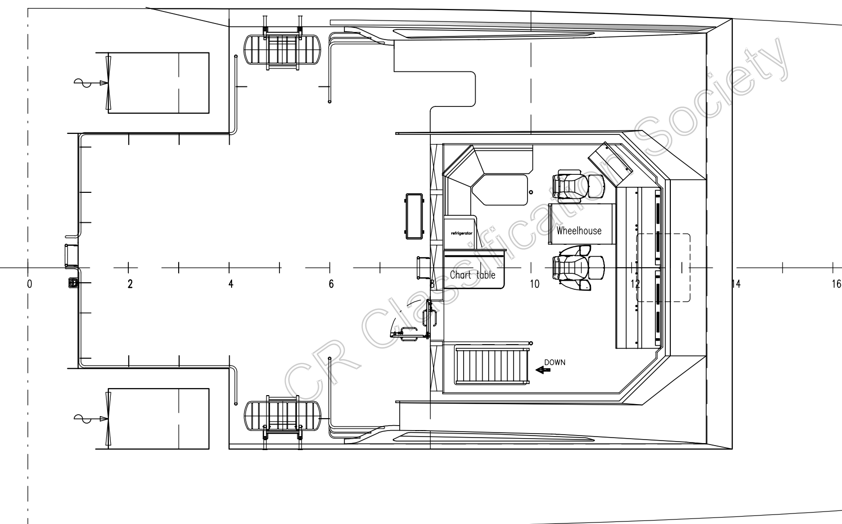
Bridge deck
